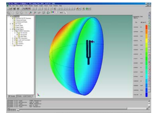
Directivity of radiated acoustic field
