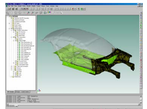
Hybrid FE-SEA structure-borne noise model of a BIW
