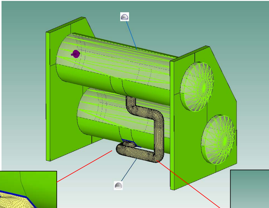
Simplified VA One model of an Industrial Chiller
